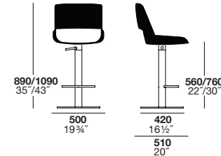
swivel O base stool 25.0033
