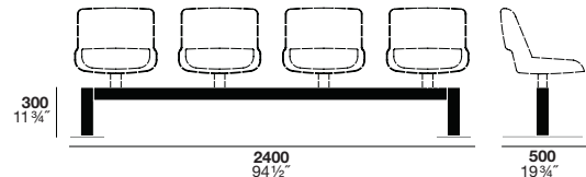
waiting area - bar 50.0001
