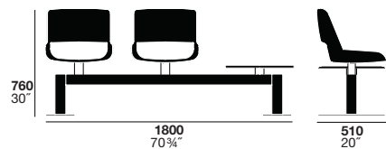
waiting area - 2 chairs + side table 50.0001/2/3
