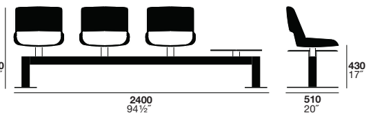
waiting area - 3 chairs + side table 50.0001/2/3
