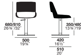
swivel O base chair 25.0032
