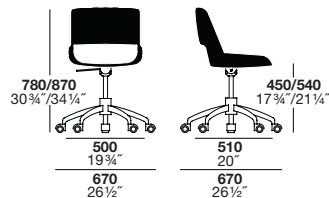
swivel 5 base chair 25.0034
