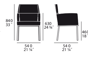
fixed armchair 10.0111
