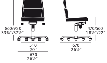
swivel armchair 10.0112
