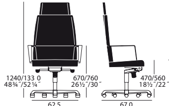
president high back armchair with headrest and armrest 10.0119
