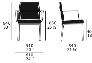
fixed armchair 10.0111
