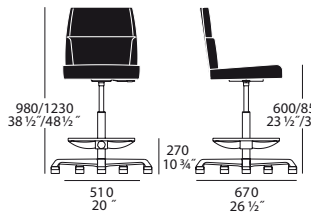
swivel stool 10.0104
