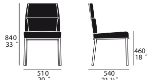
fixed chair 10.0110
