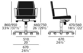
swivel chair with armrest 10.0108
