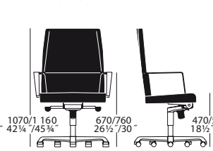
president high back armchair with armrest 10.0118
