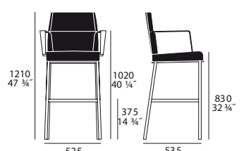
fixed stool with armrest 10.0105
