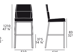
fixed stool 10.0106
