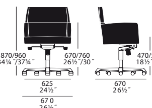
president low back armchair 10.0116
