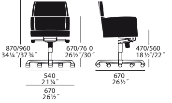
swivel armchair 10.0112
