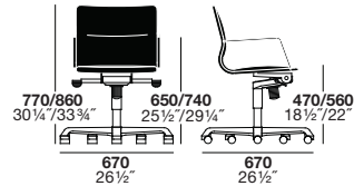
low back swivel chair - comfort 10.0170C
