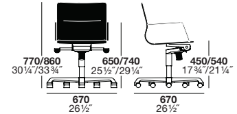
low back swivel chair 10.0170
