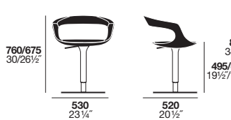
swivel chair 10.0406
